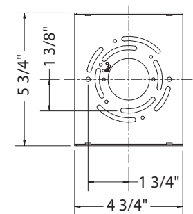
WALL PLATE
